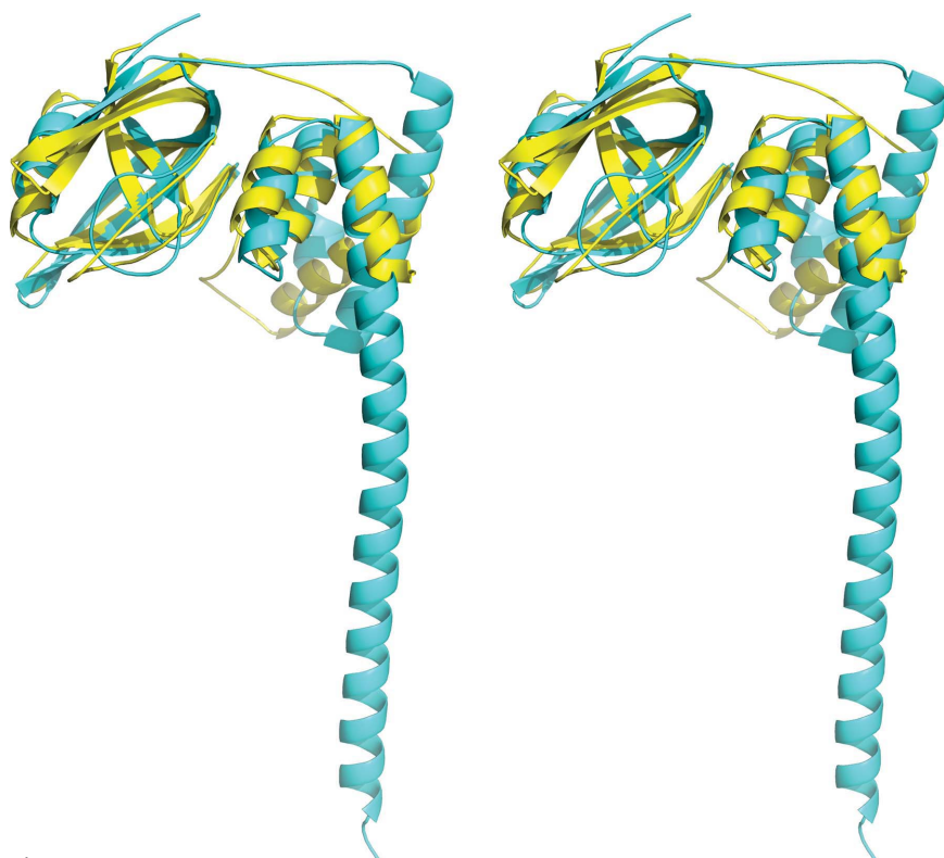
Figure 4 Comparison of the backbone trace of Lon-N245 (blue) with the hypothetical B. parapertussis protein BB1347 (yellow).
