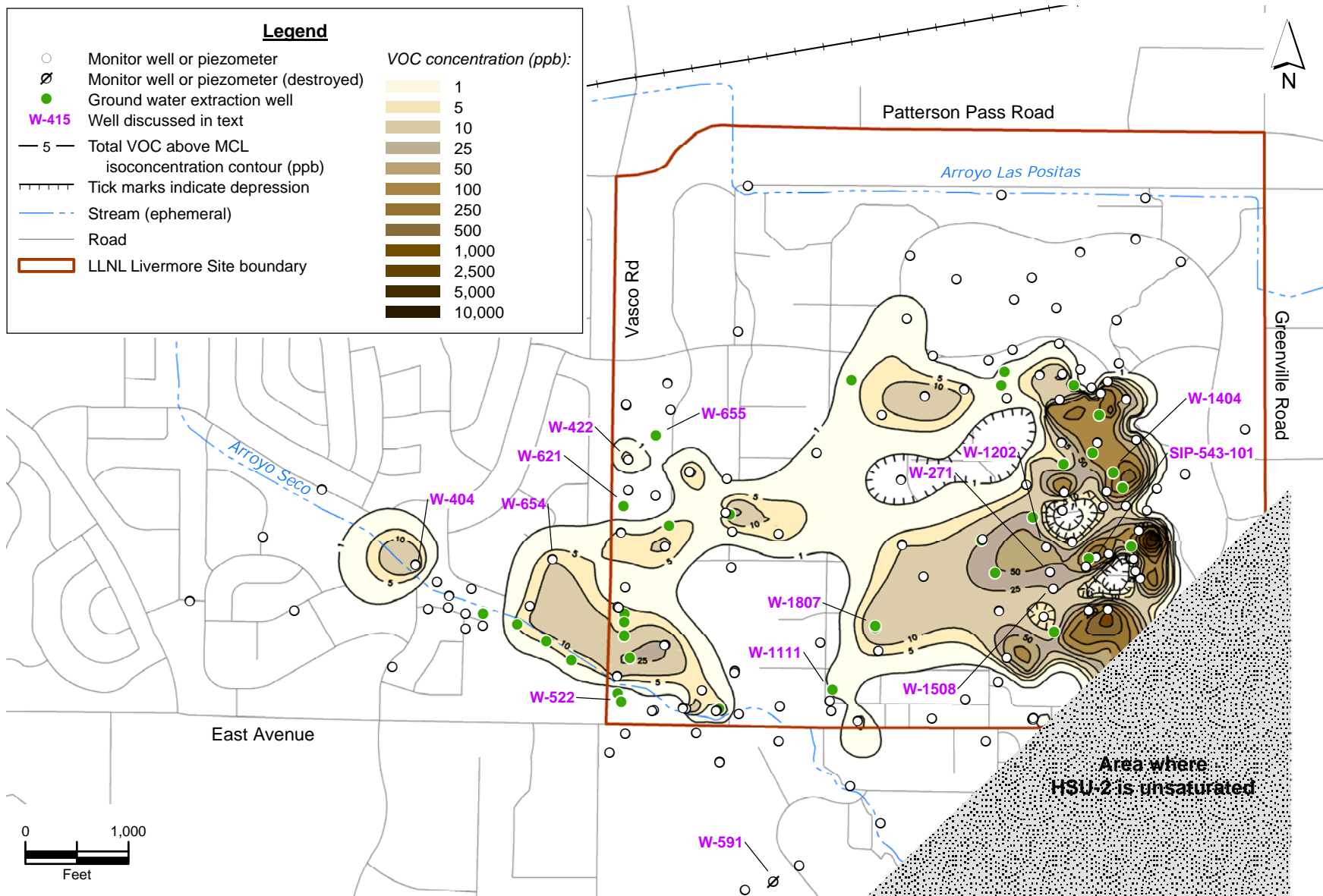
Figure 11. Isoconcentration contour map of total VOCs above MCLs from 192 wells completed within HSU-2, fourth quarter 2006 (or the next most recent data), and supplemented with soil chemistry data from 80 borehole locations.
