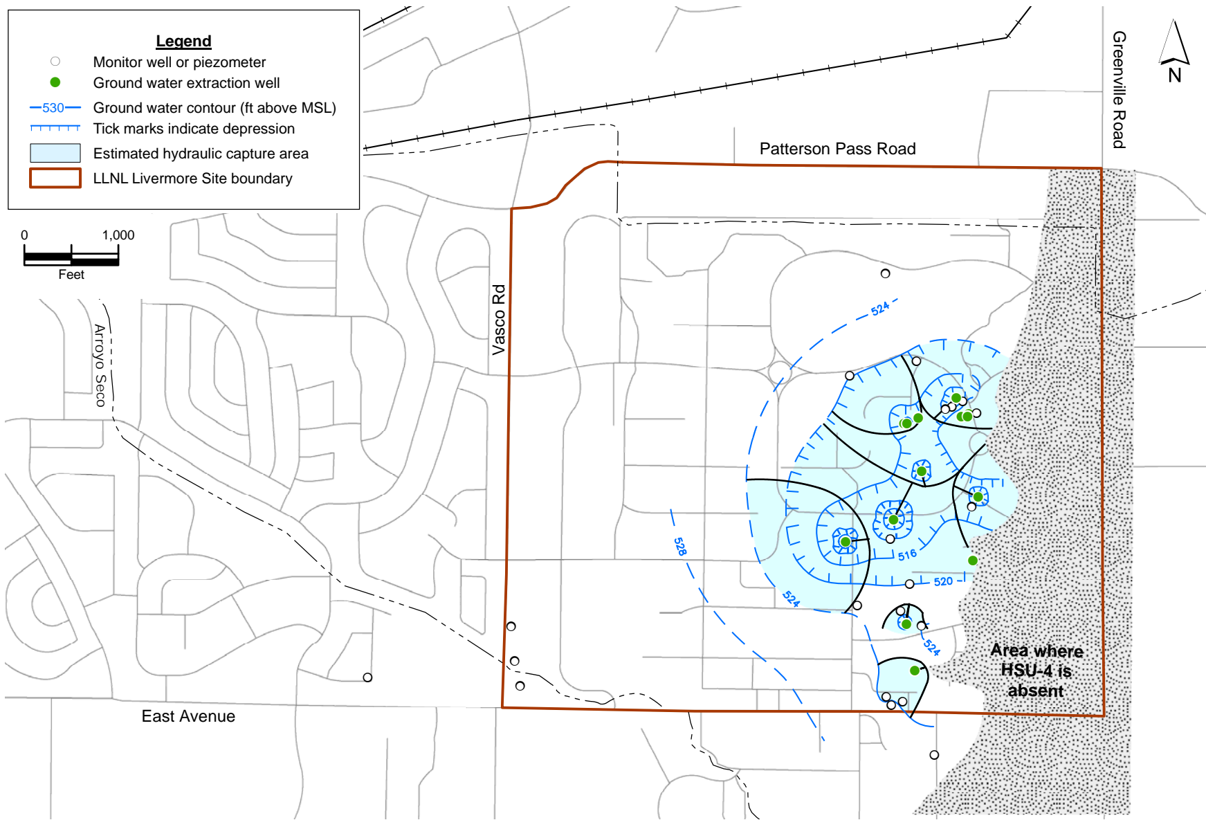
Figure 8. Ground water elevation contour map based on 39 wells completed within HSU-4 showing estimated hydraulic capture areas, LLNL and vicinity, December 2006.
