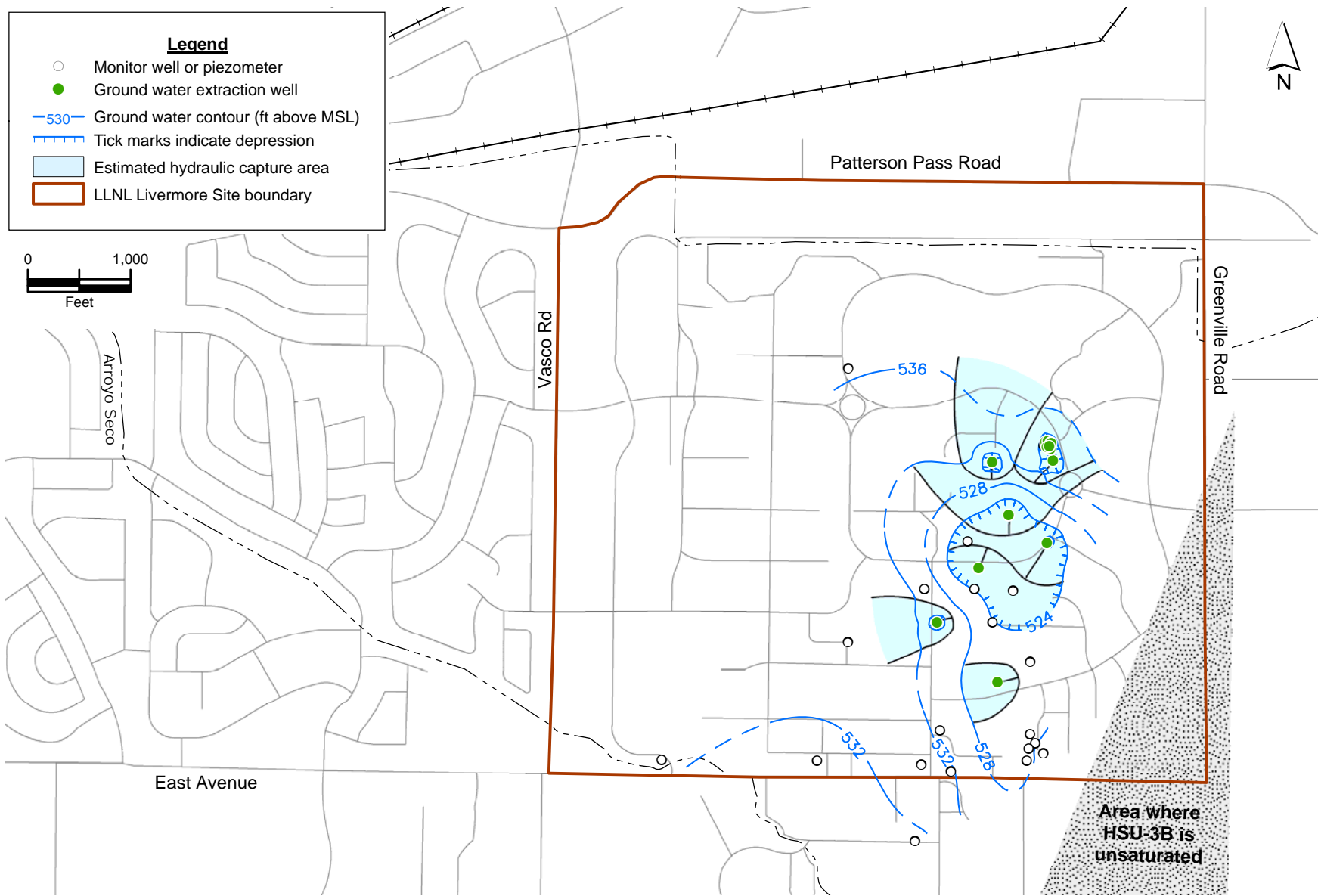
Figure 7. Ground water elevation contour map based on 34 wells completed within HSU-3B showing estimated hydraulic capture areas, LLNL and vicinity, December 2006.
