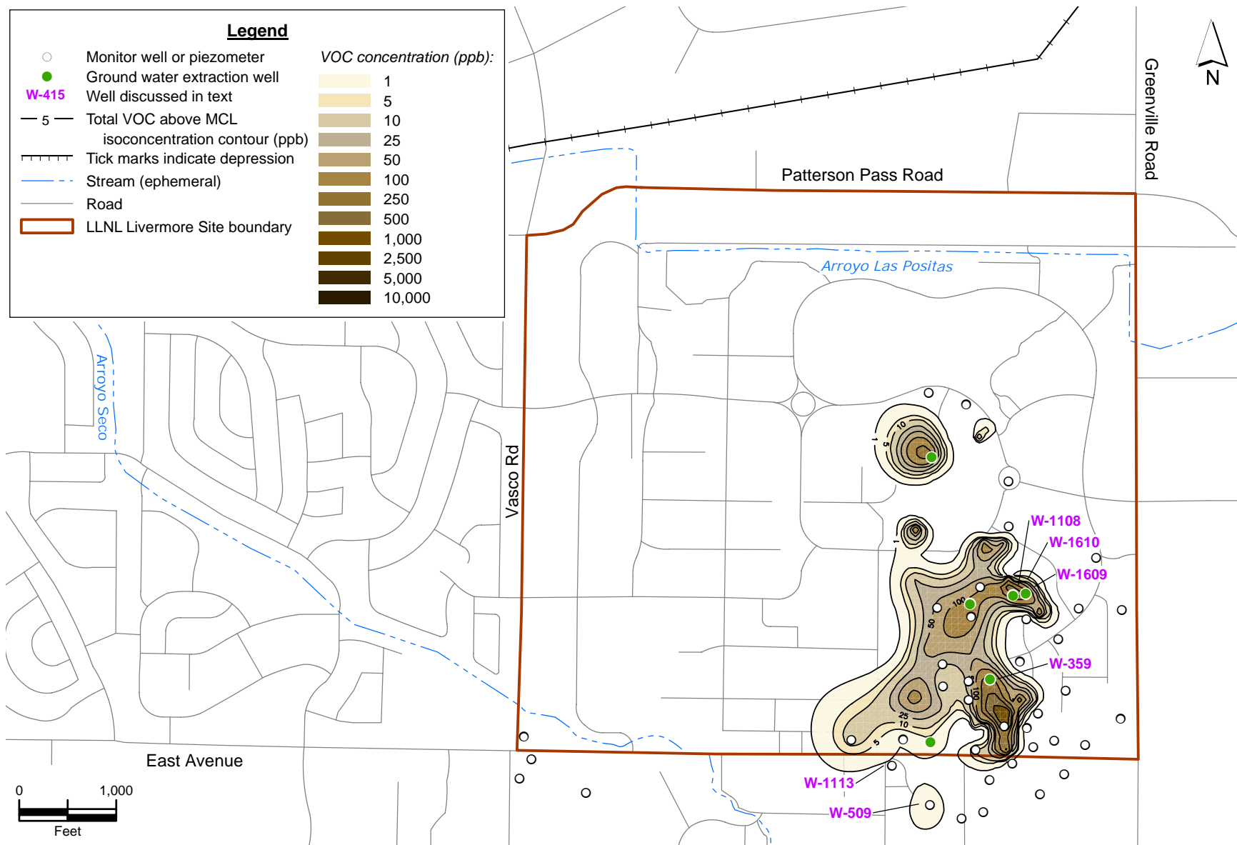
Figure 15. Isoconcentration contour map of total VOCs above MCLs from 54 wells completed within HSU-5, fourth quarter 2006 (or the next most recent data), and supplemented with soil chemistry data from 86 borehole locations.
