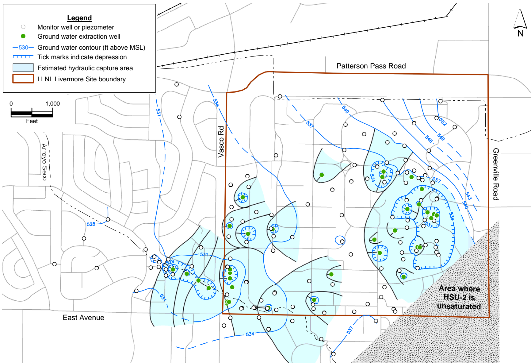
Figure 5. Ground water elevation contour map based on 182 wells completed within HSU-2 showing estimated hydraulic capture areas, LLNL and vicinity, December 2006.
