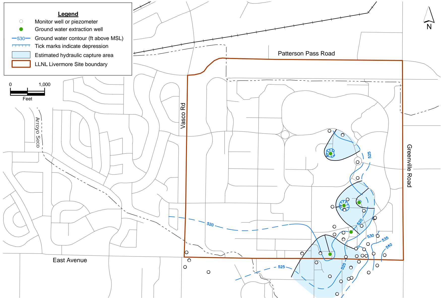
Figure 9. Ground water elevation contour map based on 51 wells completed within HSU-5 showing estimated hydraulic capture areas, LLNL and vicinity, December 2006.
