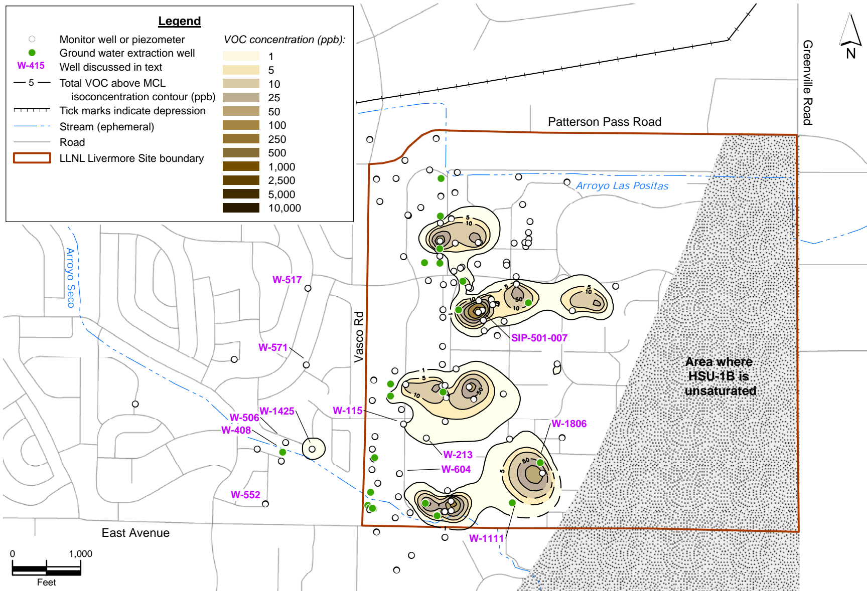
Figure 10. Isoconcentration contour map of total VOCs above MCLs from 135 wells completed within HSU-1B, fourth quarter 2006 (or the next most recent data), and supplemented with soil chemistry data from 38 borehole locations.
