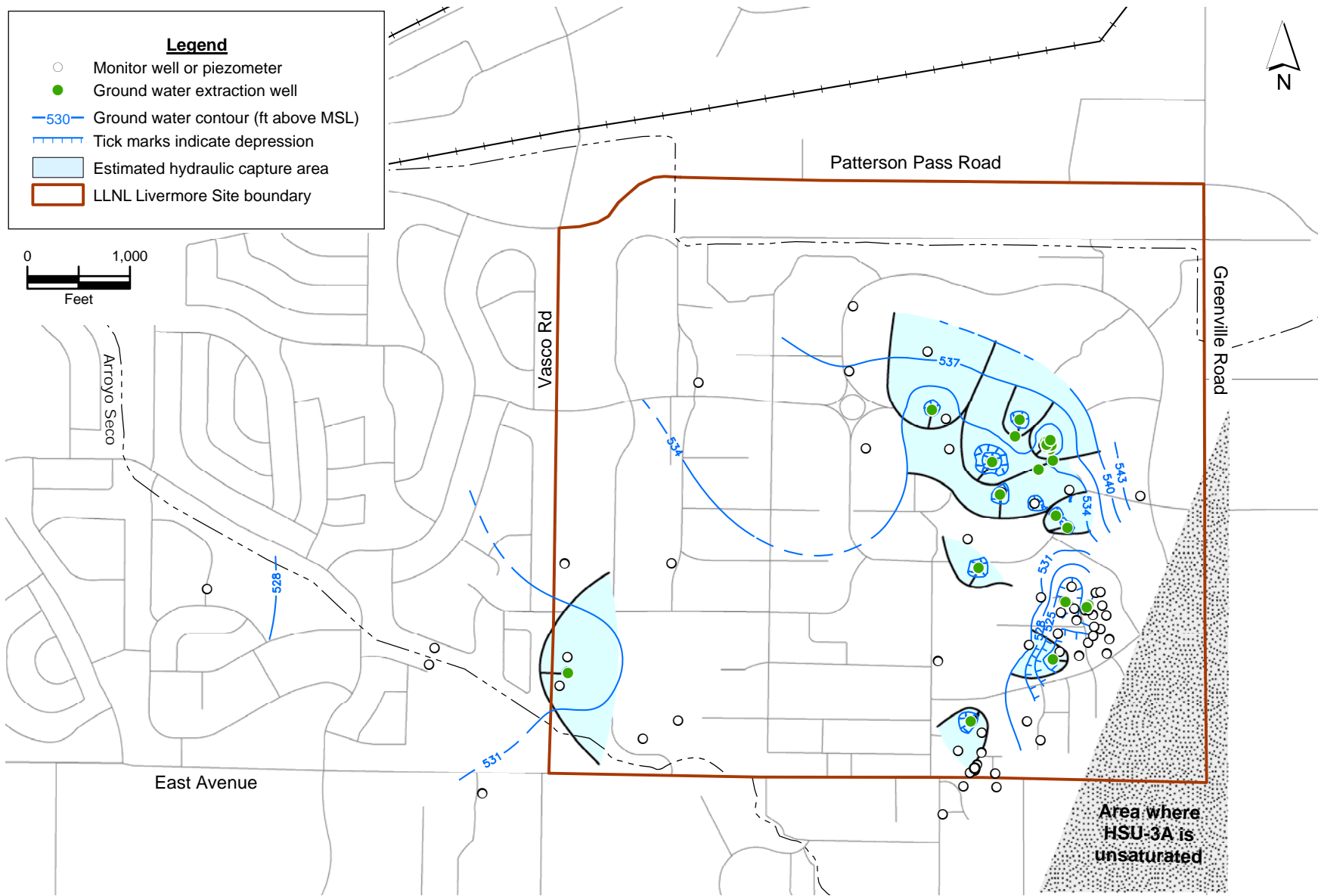
Figure 6. Ground water elevation contour map based on 102 wells completed within HSU-3A showing estimated hydraulic capture areas, LLNL and vicinity, December 2006.
