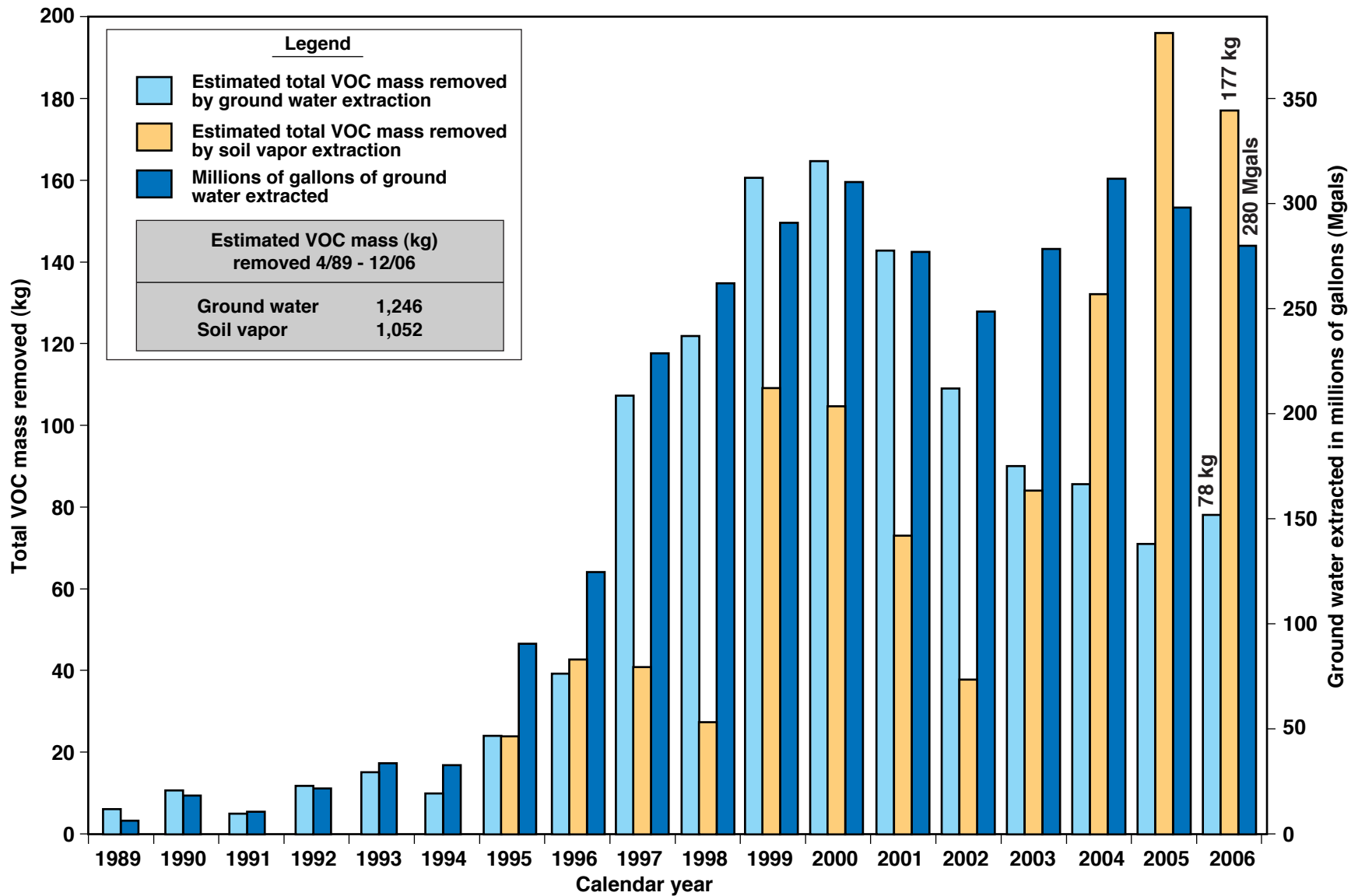
Figure 3. Estimated total VOC mass removed from the Livermore Site subsurface since 1989. All values are rounded numbers.
