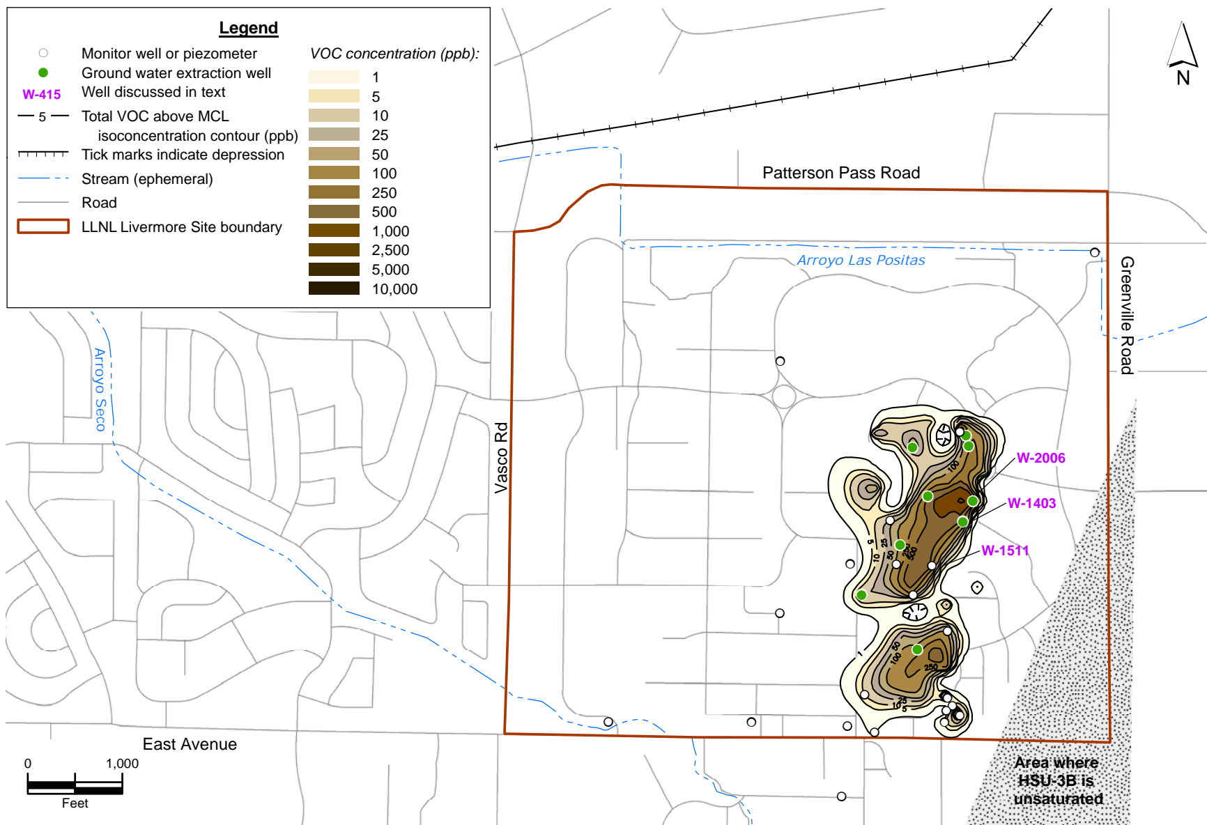
Figure 13. Isoconcentration contour map of total VOCs above MCLs from 39 wells completed within HSU-3B, fourth quarter 2006 (or the next most recent data), and supplemented with soil chemistry data from 108 borehole locations.
