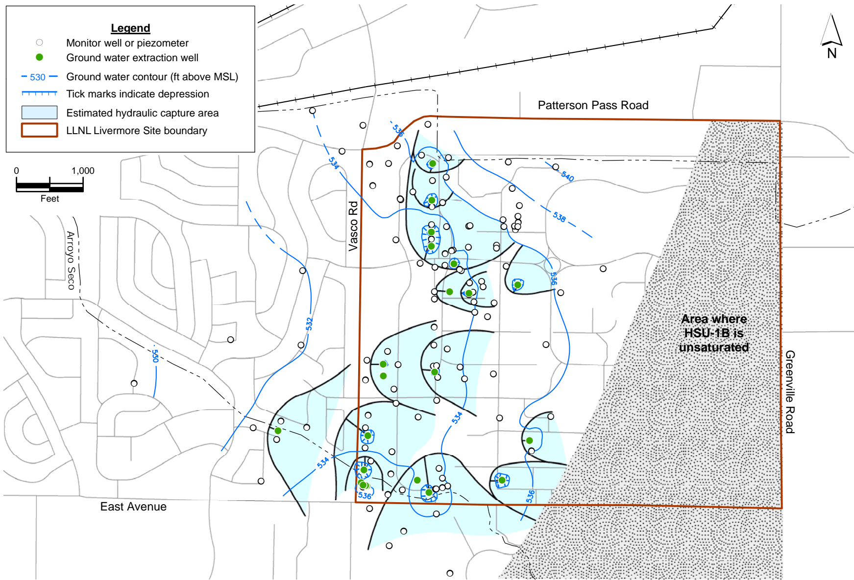
Figure 4. Ground water elevation contour map based on 135 wells completed within HSU-1B showing estimated hydraulic capture areas, LLNL and vicinity, November 2006.
