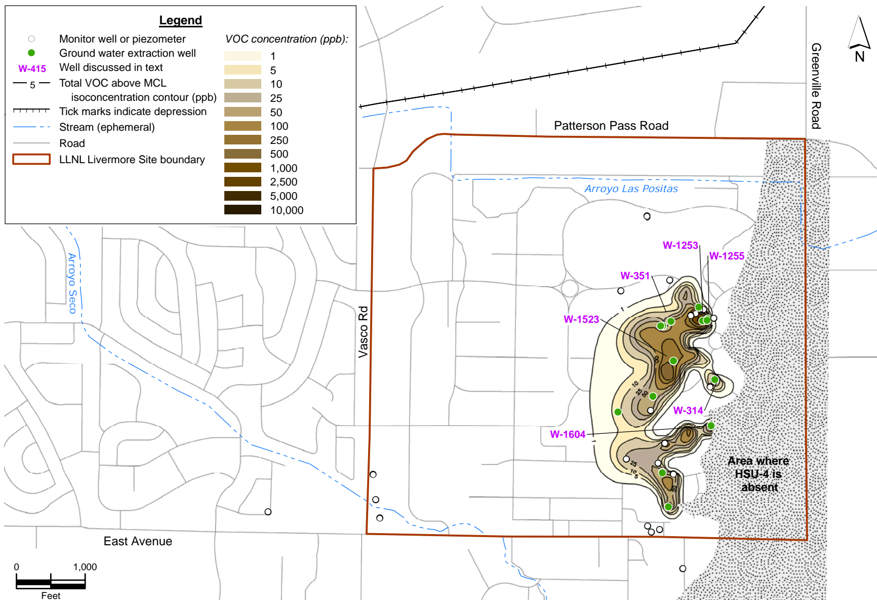
Figure 14. Isoconcentration contour map of total VOCs above MCLs from 41 wells completed within HSU-4, fourth quarter 2006 (or the next most recent data), and supplemented with soil chemistry data from 55 borehole locations.
