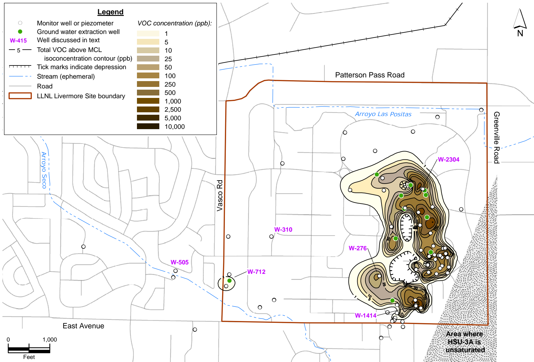
Figure 12. Isoconcentration contour map of total VOCs above MCLs from 103 wells completed within HSU-3A, fourth quarter 2006 (or the next most recent data), and supplemented with soil chemistry data from 141 borehole locations.
