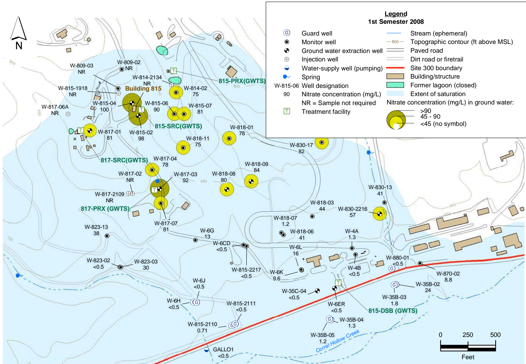
Figure 2.4-11. High Explosives Process Area map showing nitrate concentrations for the Tnbs 2 HSU.
