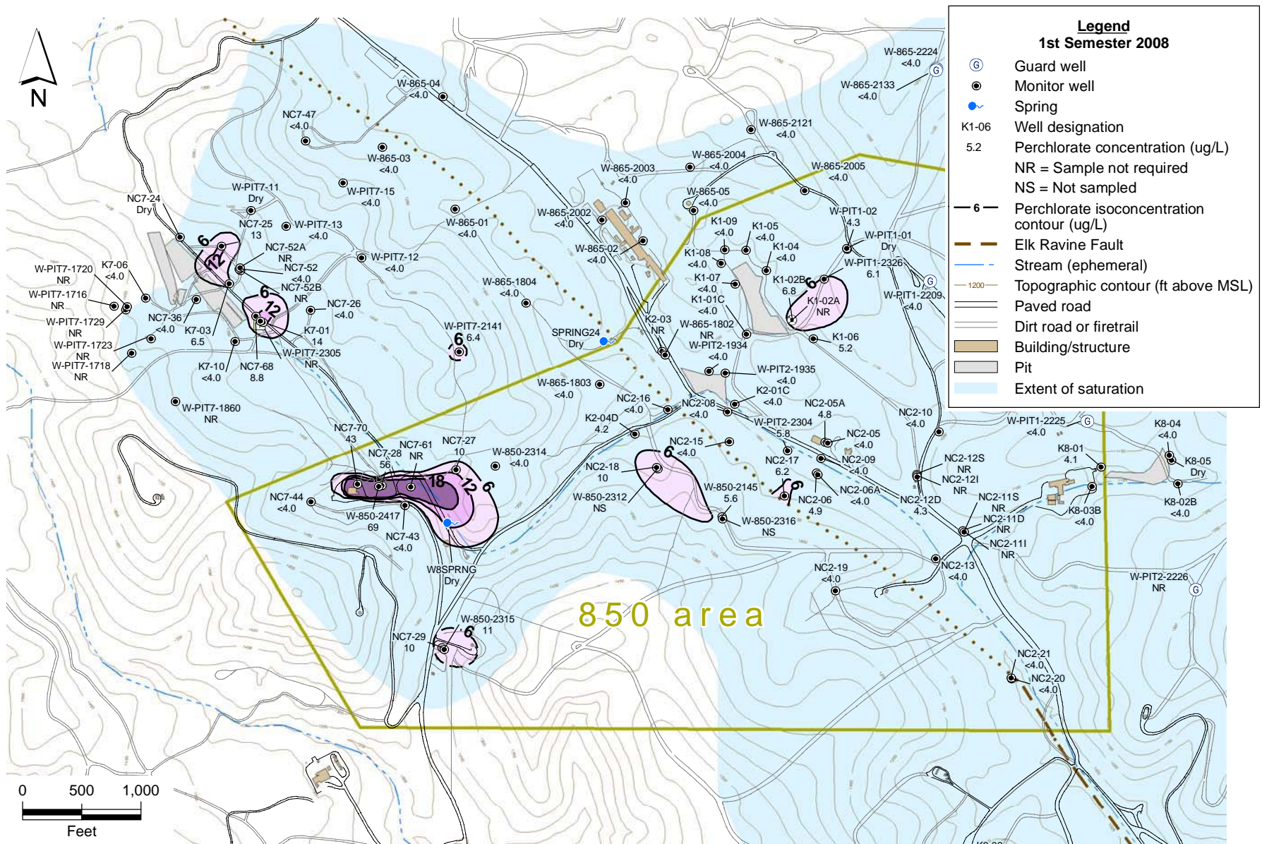
Figure 2.5-11. Building 850 area perchlorate isoconcentration contour map for the Tnbs 1 /Tnbs 0 HSU.
