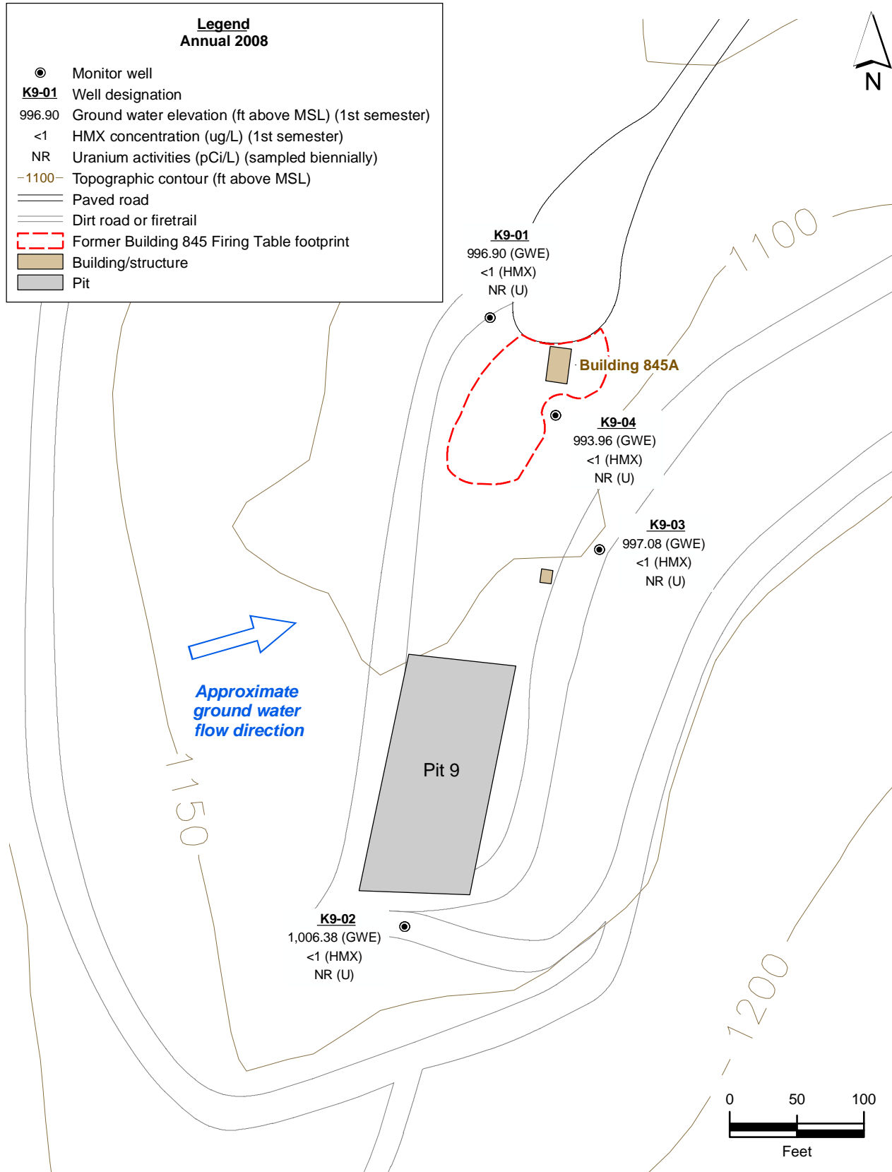
Figure 2.8-3. Building 845 Firing Table and Pit 9 Landfill site map showing monitor well locations, ground water elevations, ground water flow direction, HMX concentrations and uranium activities in the Tnsc 0 HSU.
