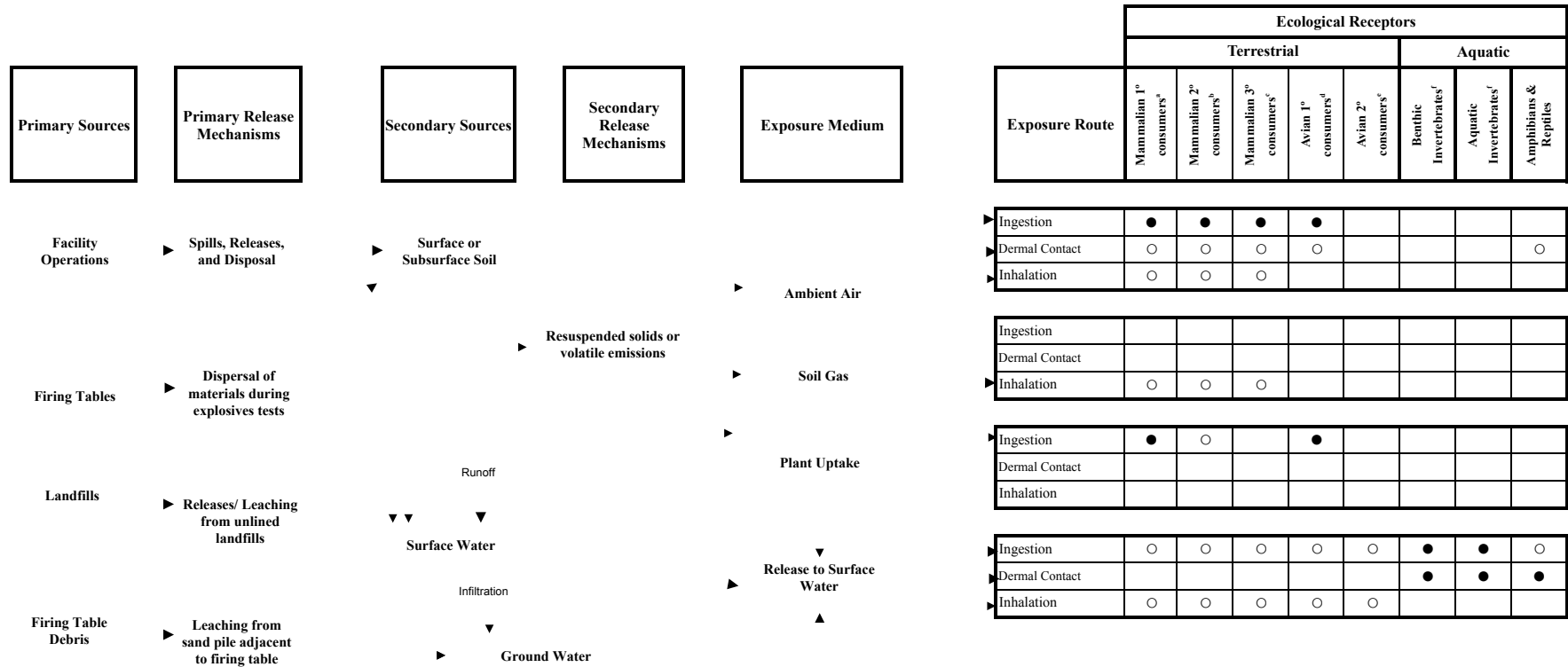
Figure 4.2-3. Generalized Conceptual Site Model for LLNL Site 300 Lawrence Livermore National Laboratory, Site 300, Livermore, California
