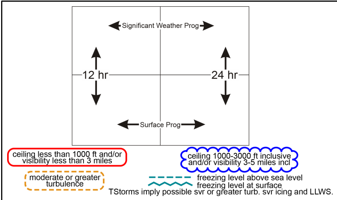
Figure 2-6 Significant Weather Prognostic Legend
