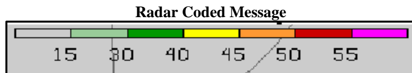
Figure 2-10 Precipitation Intensity Levels
