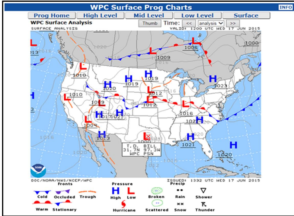
Figure 2-22 Surface Analysis Chart for Questions 6-8
