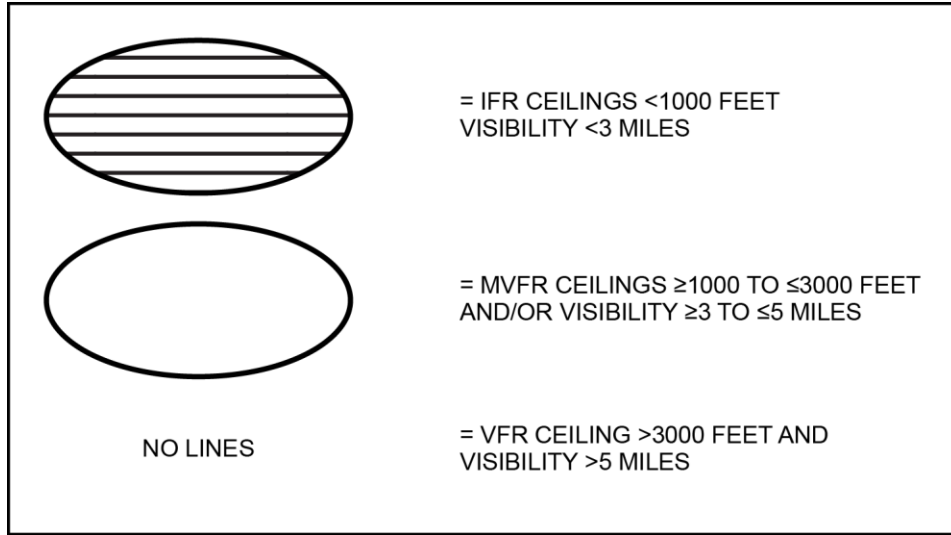
Figure 2-18 Weather Depiction Chart Legend
