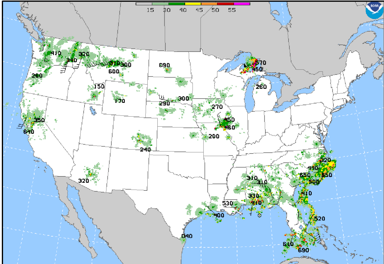
Figure 2-24 Radar Summary Chart for Questions 14-17
