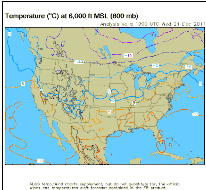
Figure E-10 ADDS Temp/Winds Chart Supplement
