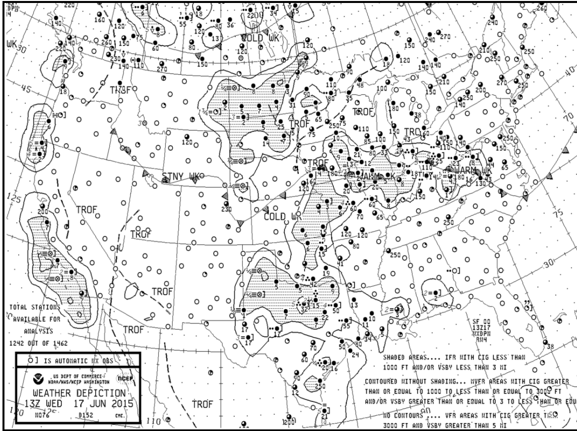
Figure E-9 Weather Depiction Chart
