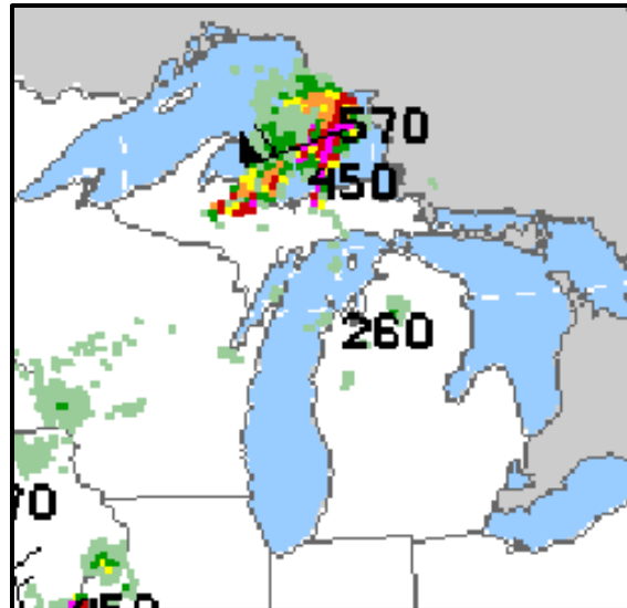
Figure 2-9 Radar Summary Chart
