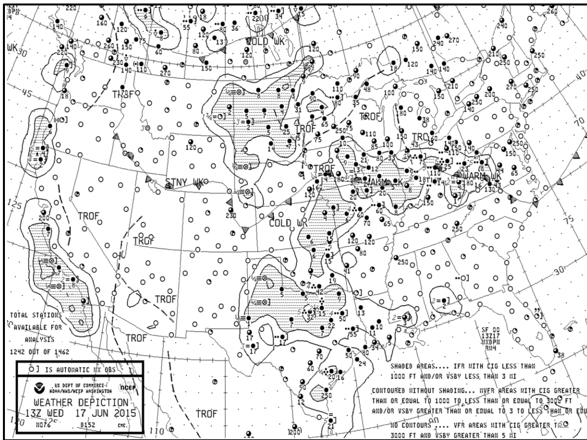
Figure 2-16 Weather Depiction Chart
