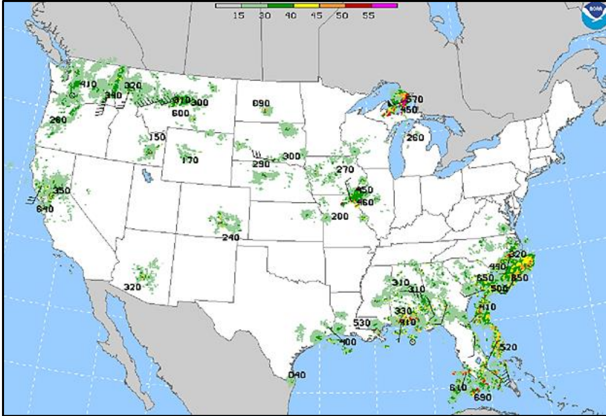
Figure 2-8 Radar Summary Chart
