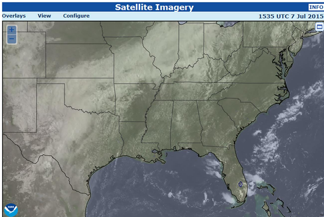
Figure 2-13 Visible Satellite Imagery
