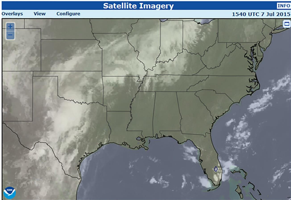
Figure 2-14 Infrared Satellite Imagery
