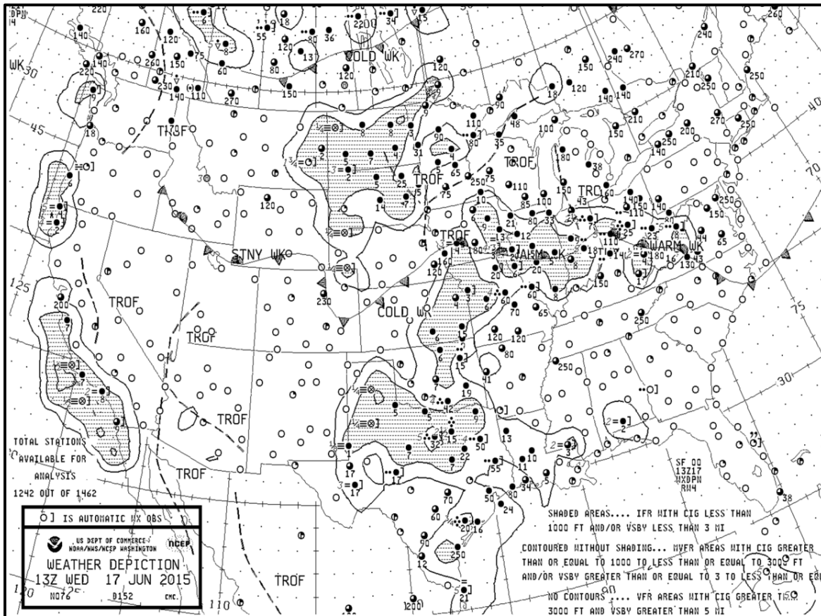
Figure 2-25 Weather Depiction Chart for Questions 26 - 29
