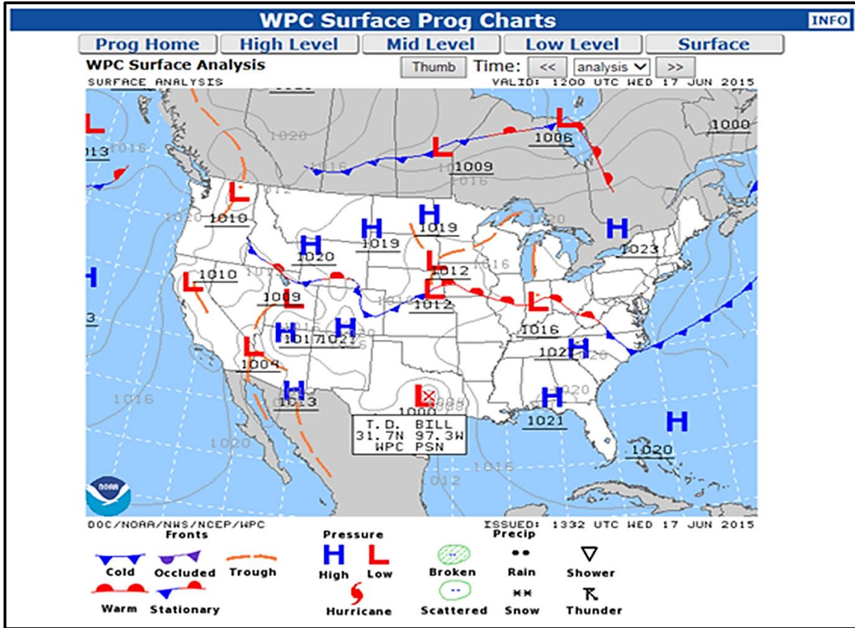
Figure E-4 Surface Analysis Chart
