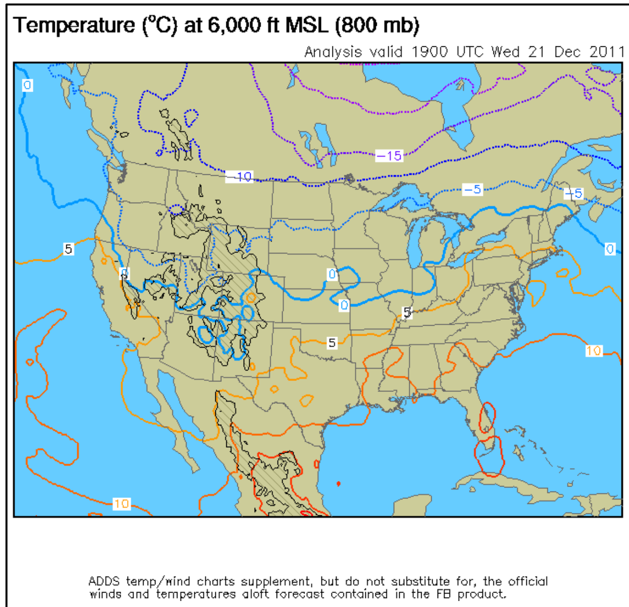
Figure 2-20 ADDS Temp/Wind Charts Supplement (2)
