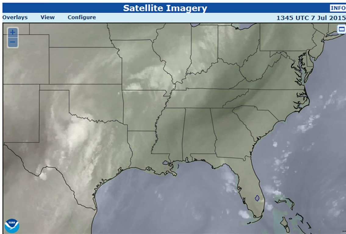
Figure 2-15 Water Vapor Imagery
