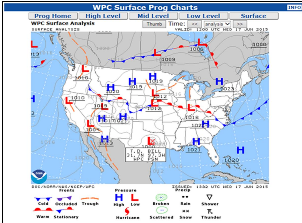
Figure 2-1 Surface Analysis Chart
