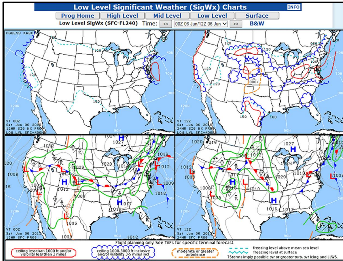
Figure 2-23 Low Level Significant Weather Prognostic Chart for Questions 9-13
