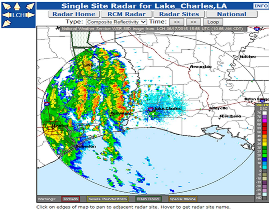
Figure 2-11 Lake Charles NEXRAD Display
