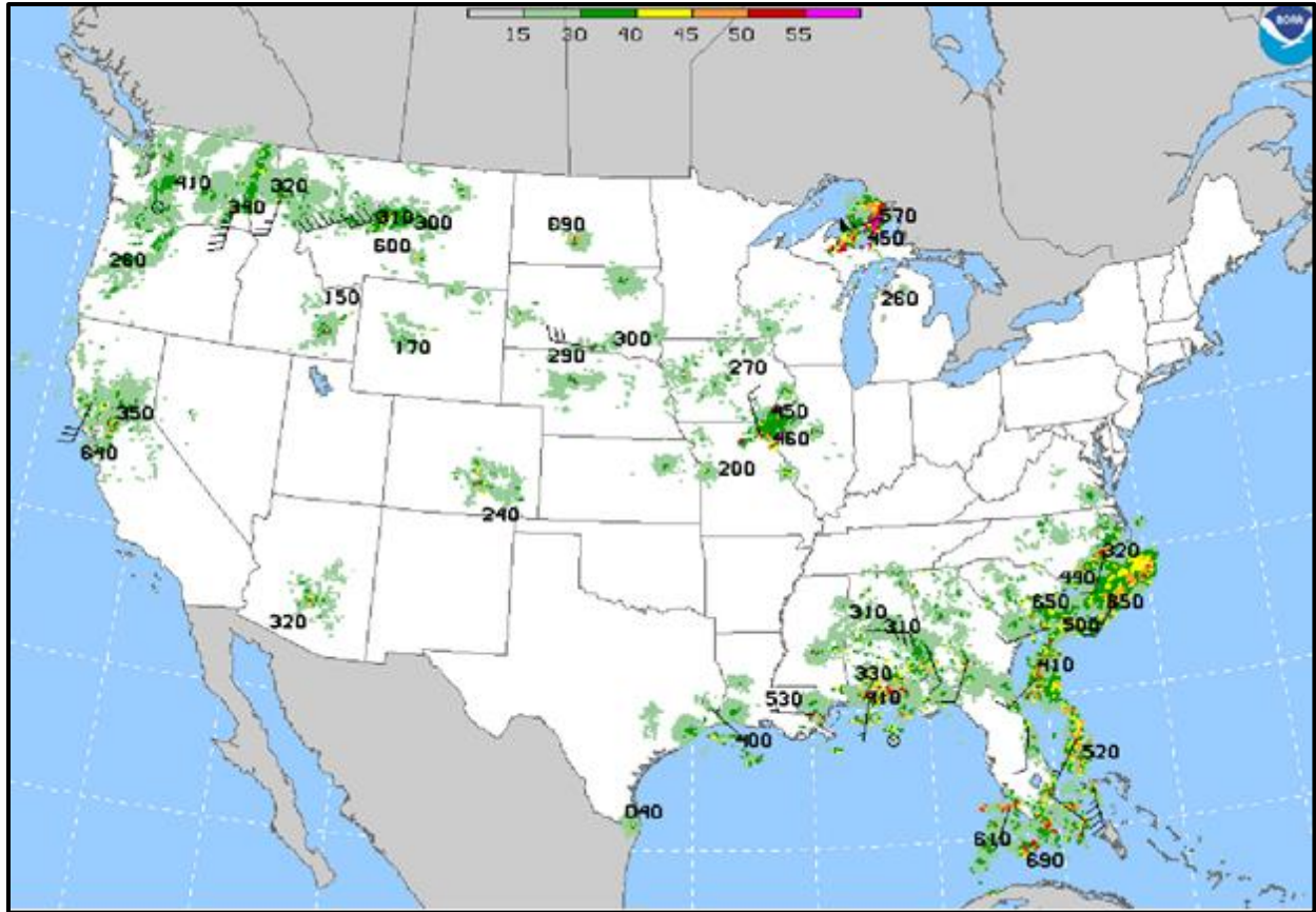
Figure E-8 Radar Summary Chart
