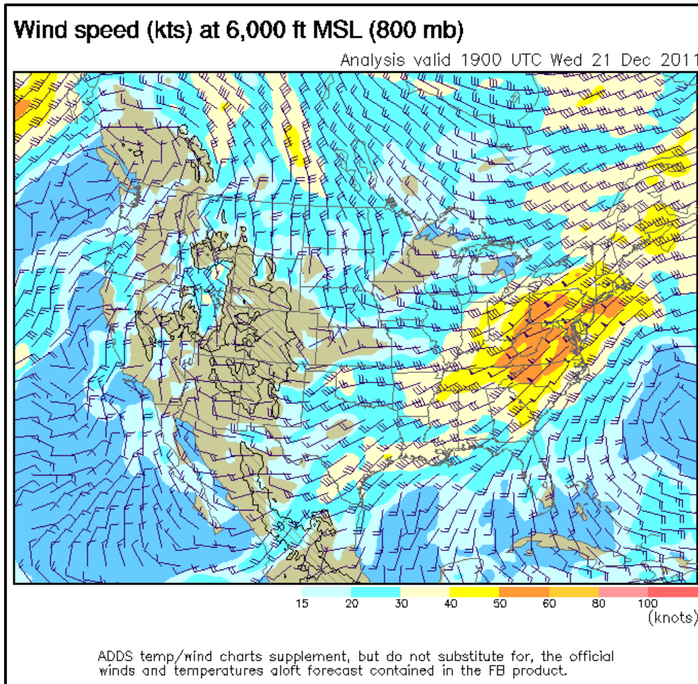
Figure 2-19 ADDS Temp/Wind Charts Supplement (1)
