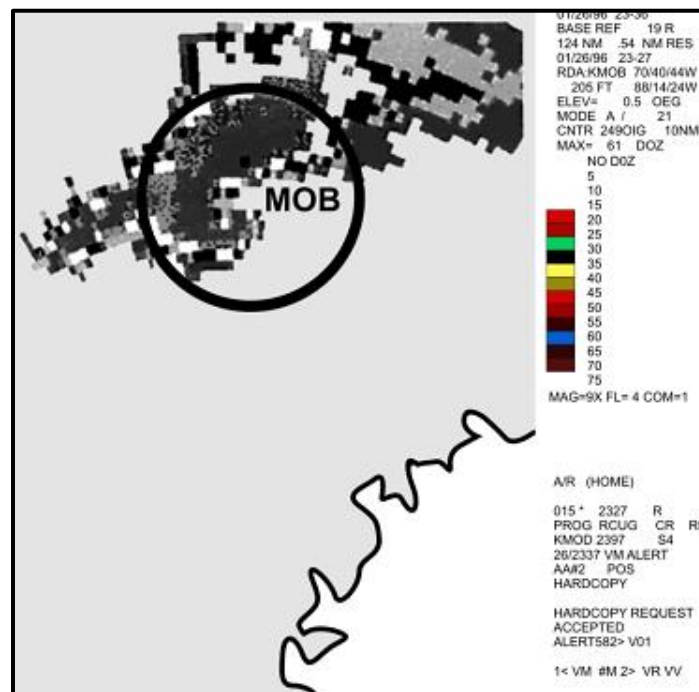
Figure 2-12 Hook Echo on NEXRAD
