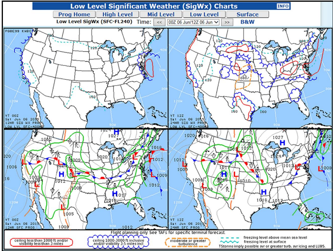
Figure E-6 Low Level Significant Weather Prognostic Chart
