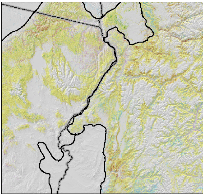
Figure 6: LANDFIRE Canopy Cover and Canopy Height for ponderosa pine – Douglas-fir systems (see Figure 2 for BpS units used). Only wildland areas are show for clarity.
