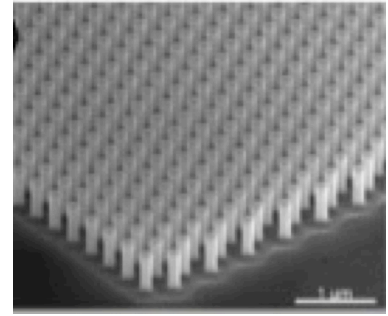
Figure 3. Nanowire arrays.
