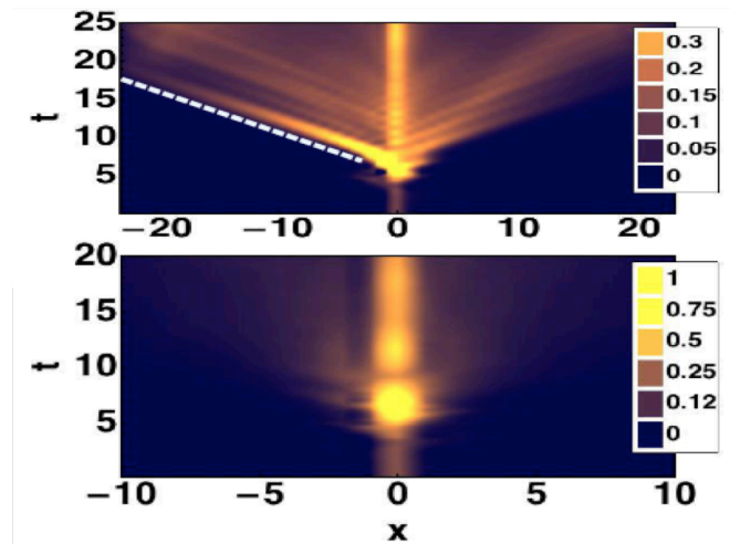
Figure 14. A polaron quasiparticle (an electron dressed by fully quantum phonons) in a nanowire is excited by an ultrafast optical pulse.
