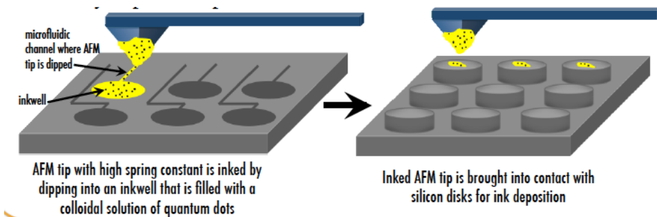
Figure 13. Dip Pen Nanolithography using a quantum dot ink.
