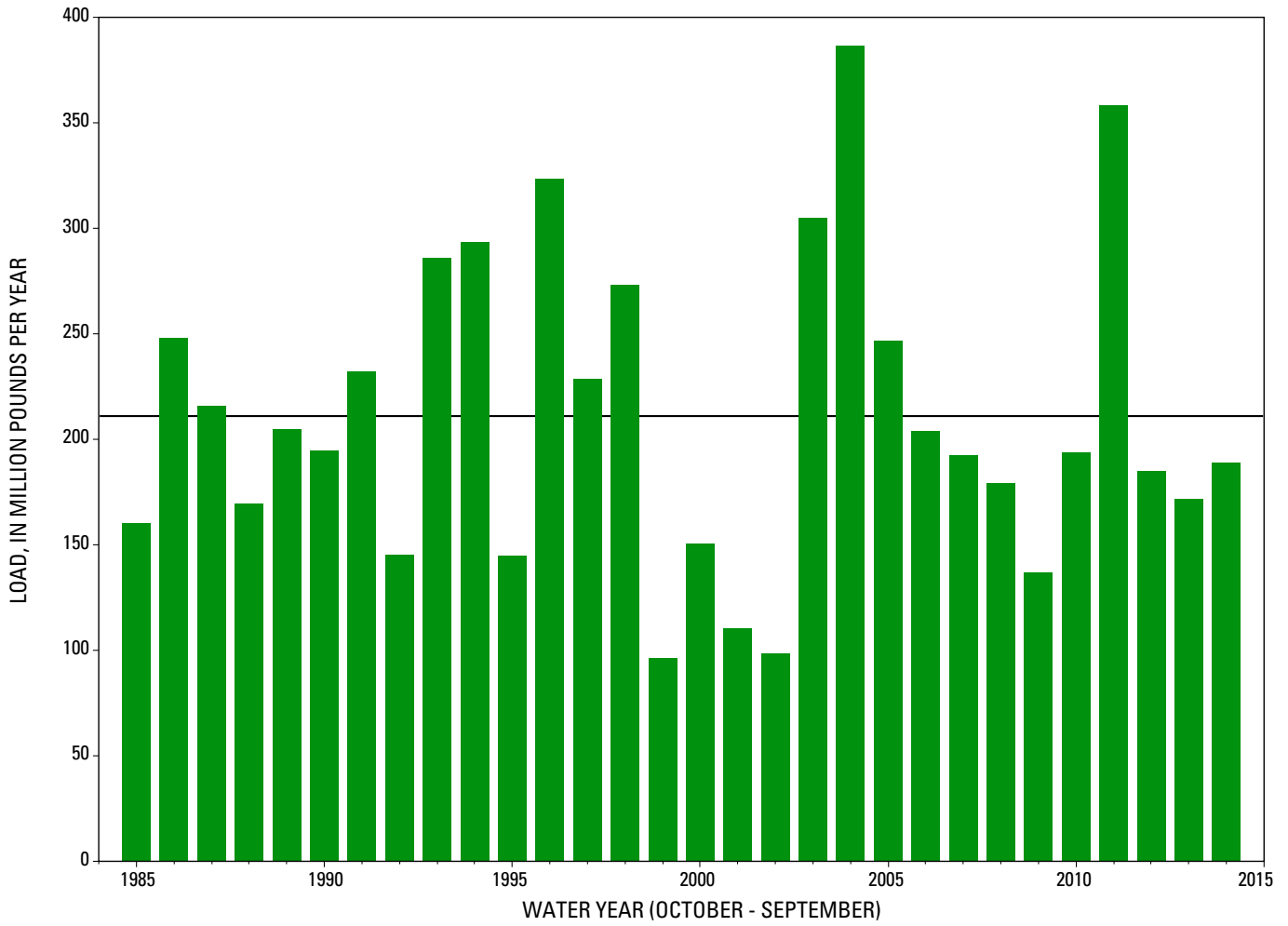
Figure 3. Combined annual total nitrogen load delivered from the nine River Input Monitoring stations to the Chesapeake Bay. Black line represents the mean annual combined load of 210 million pounds per year.
