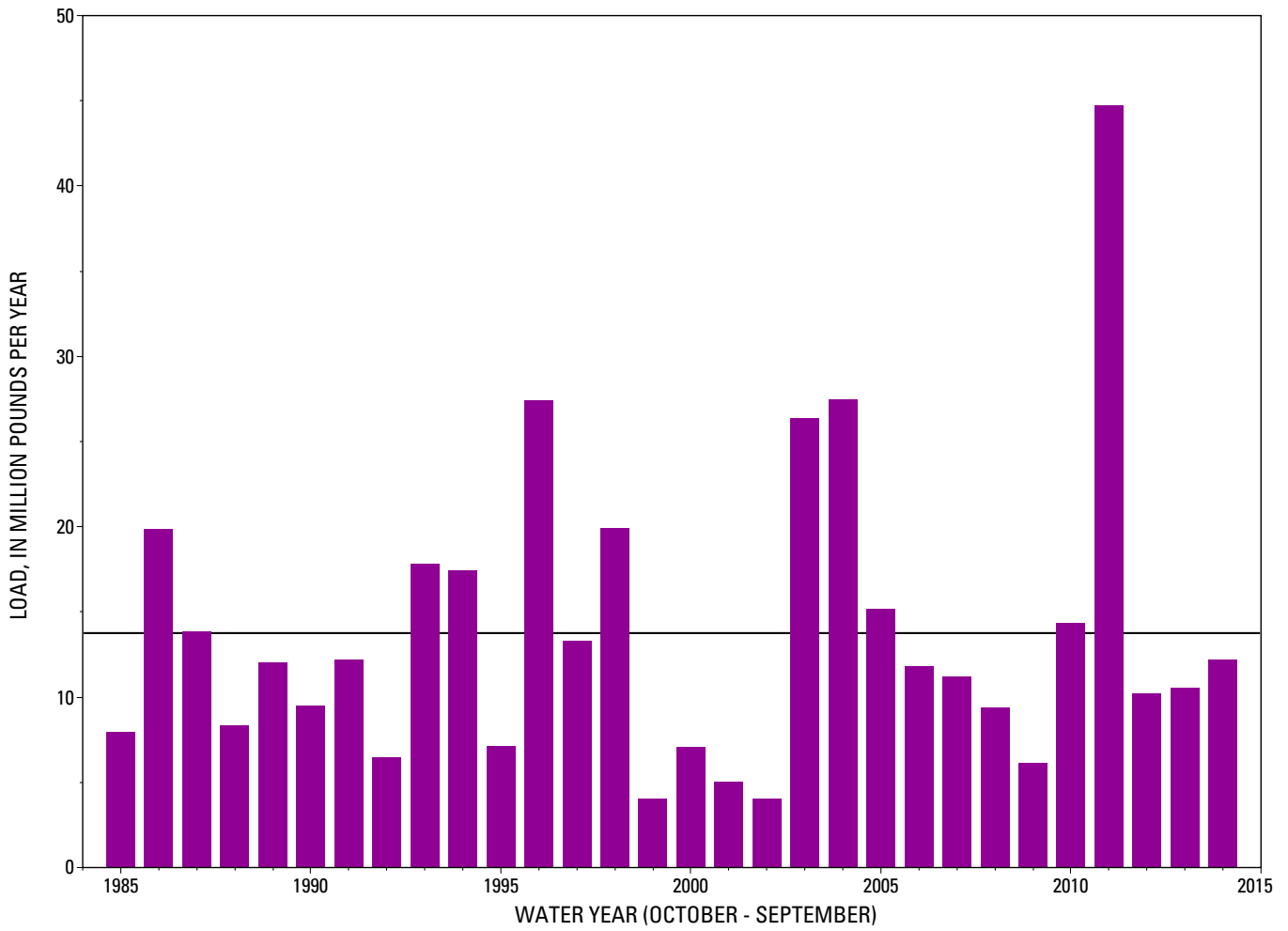
Figure 4. Combined annual total phosphorus load delivered from the nine River Input Monitoring stations to the Chesapeake Bay. Black line represents the mean annual combined load of 13.7 million pounds per year.
