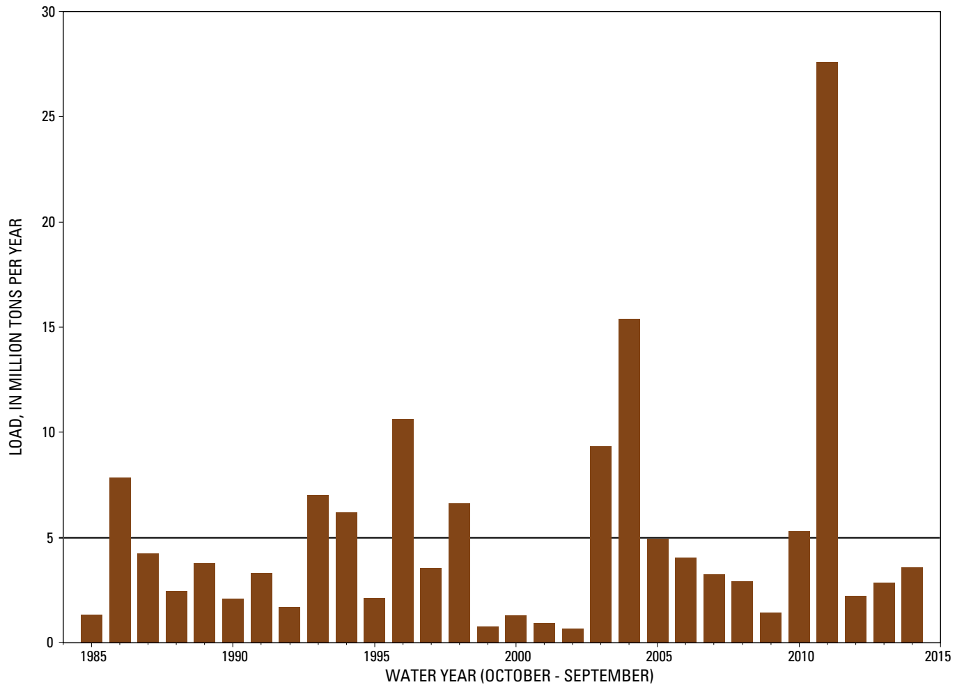
Figure 5. Combined annual suspended-sediment load delivered from the nine River Input Monitoring stations to the Chesapeake Bay. Black line represents the mean annual combined load of 4.99 million tons per year.
