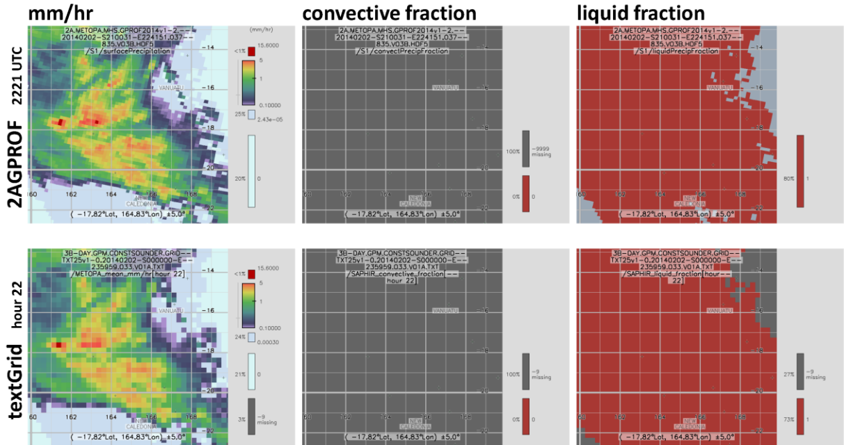
Fig. 1. Comparisons of hour 22 of the sounder gridded text product with the 2A GPROF retrieval for that time period. Figure shows precipitation rate, convective fraction (currently all missing values), and the liquid fraction.
