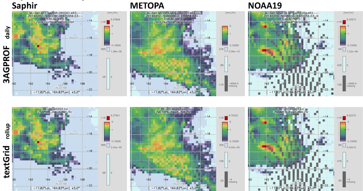
Fig. 2. Comparison of the textgrid with daily L3 GPROF gridded products. This figure contains the precipitation information from three cross-track scanning radiometers (sounders) over the same system both from the gridded text product and the L3 GPROF gridded HDF5 full product.
