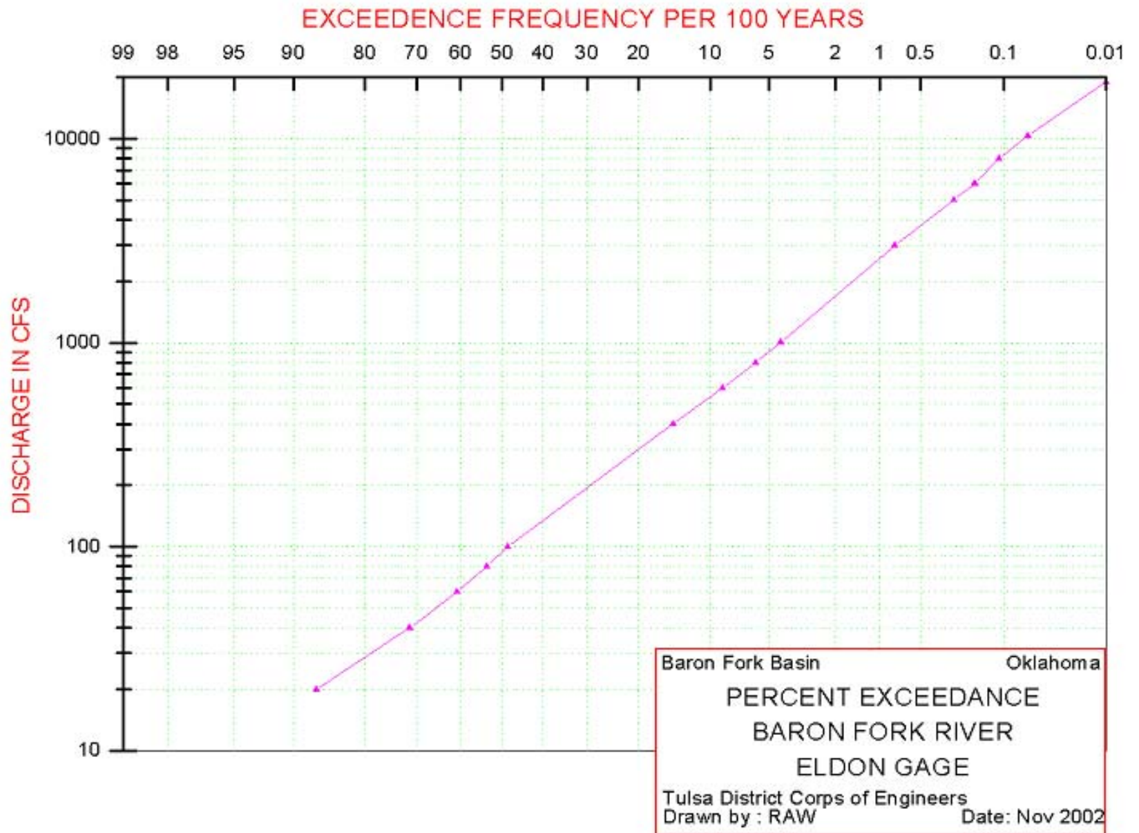
Figure 4-1. Percent Exceedance Curve.
