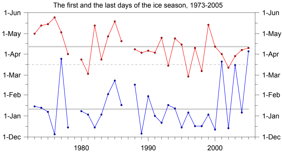
Fig. 5. The first and last days of the ice season, 1973-2005. The gray solid horizontal lines are the mean dates for these two variables. The dashed line (March 15) is used as a threshold to calculate the ice retreat index. No ice was present in the box in 1979 and 1987.
