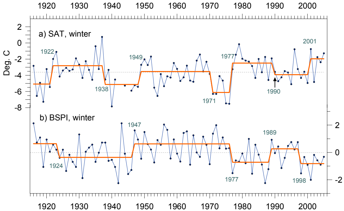
Fig. 1. Mean winter (DJFM) a) surface air temperatures in St. Paul, Pribilof Islands and b) Bering Sea pressure index. The dashed line for the top graph indicates the mean SAT value of -3.62^{\circ}\text{C} for the base period, 1961-2000. Positive (negative) values of BSPI suggest anticyclonic (cyclonic) conditions in the Bering Sea. The stepwise functions (orange lines) characterize regime shifts in the level of fluctuations of the variables. Shift points were calculated using the sequential method (Rodionov 2004), with the cutoff length of 10 years, significance level of 0.2, and Huber weight parameter of 1. The latter reduces the effect of “outliers”, if they exceed one standard deviation from the mean value of the corresponding regime.
