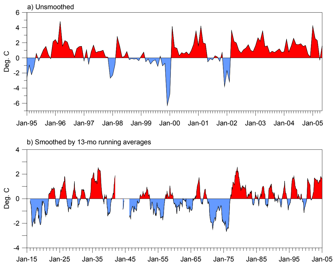
Fig. 2. Mean monthly surface air temperatures anomalies in St. Paul, Pribilof Islands, a) unsmoothed, January 1995 through May 2005, and b) smoothed by 13-mo running averages and referred to the central month of the window, January 1916 through January 2005. The base period for calculating anomalies is 1961-2000.
