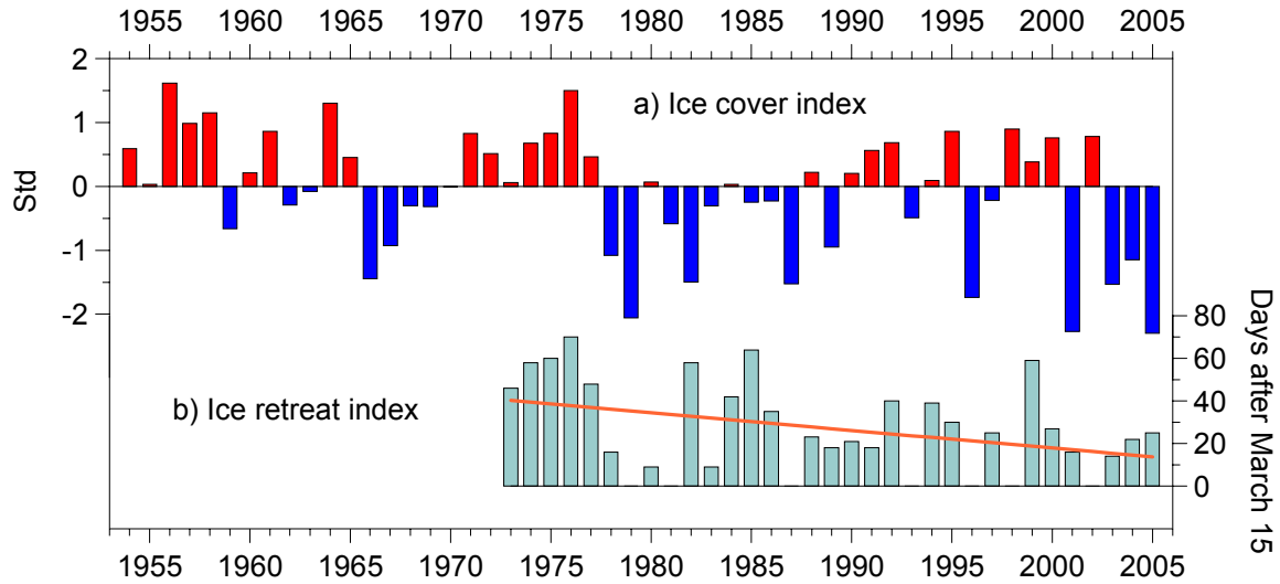
Fig. 3. a) Ice cover index, 1954-2005, and b) ice retreat index and its linear trend (orange line), 1973-2005.
