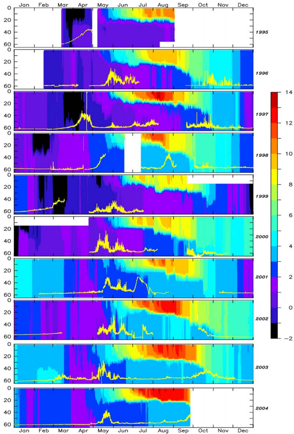
Fig. 7. Contours of temperature measured at Mooring 2, 1995-2004. The coldest temperature (black) occurred when ice was over the mooring. The yellow line is fluorescence measured at ~11m. Note that early blooms are associated with the presence of ice.
