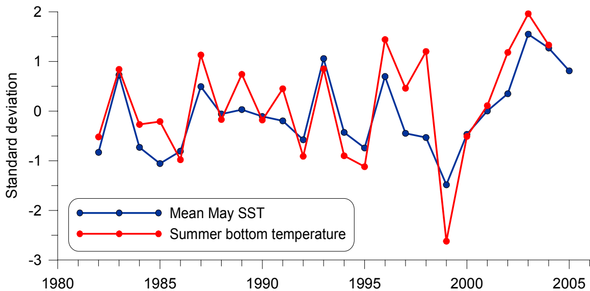
Fig. 8. The MaySST index and mean summer bottom temperature in the southeastern Bering Sea, 1982-2005.
