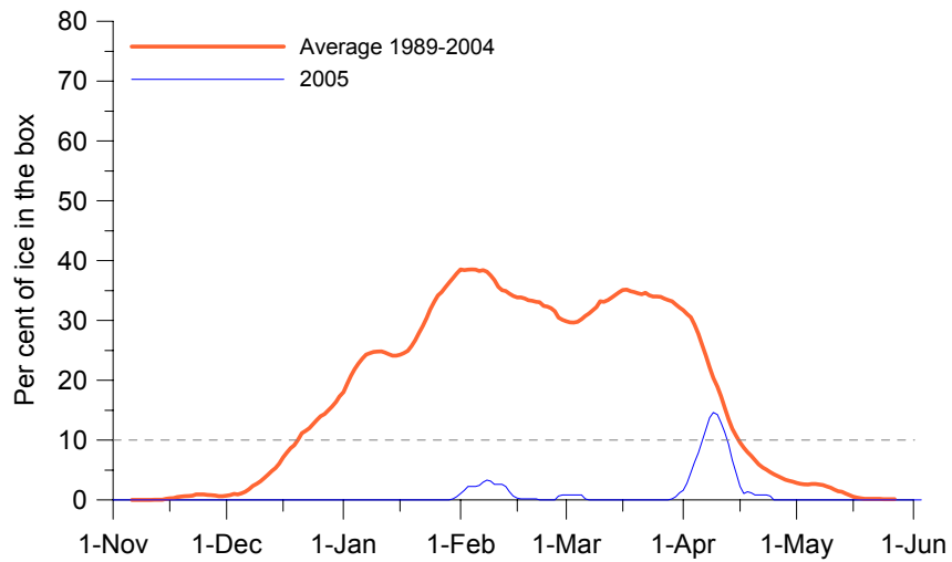
Fig. 4. Percentage of ice cover in the 2° x 2° box (56-58°N, 163-165°W) during the winter of 2005.
