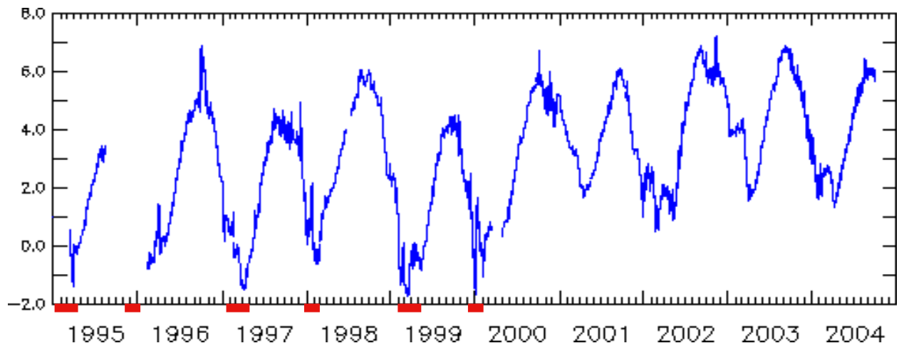
Fig. 6. Depth integrated temperature at Mooring 2. The red lines at the bottom of the plot indicate when ice was present over the mooring.
